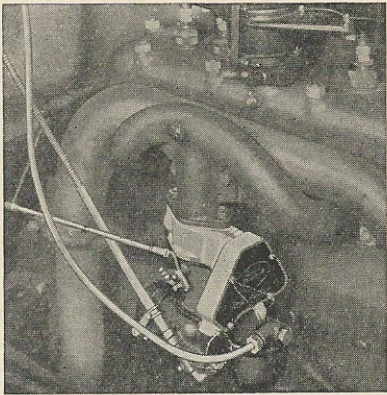
This view shows the Handy in position, between the carburetor and the intake manifold of the new Ford Truck Motor.
